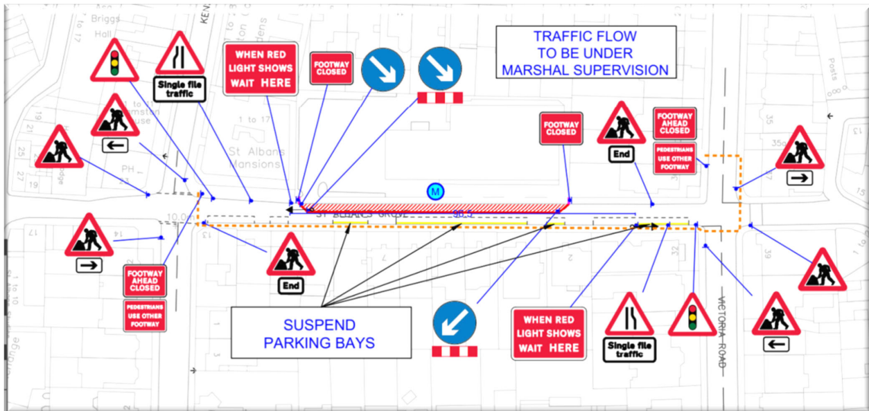
Traffic Management Plan for Tower Crane Installation 29th/30th of June
